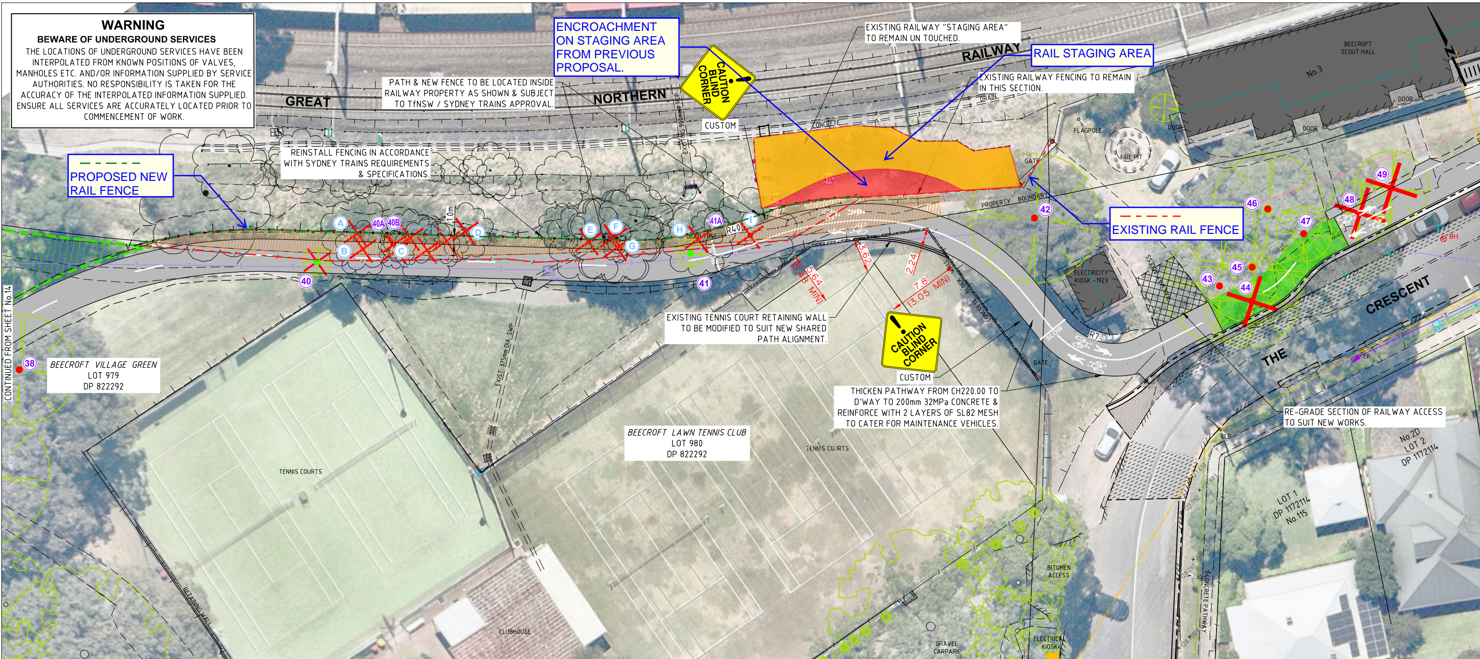
PLAN SCALE 1:200
