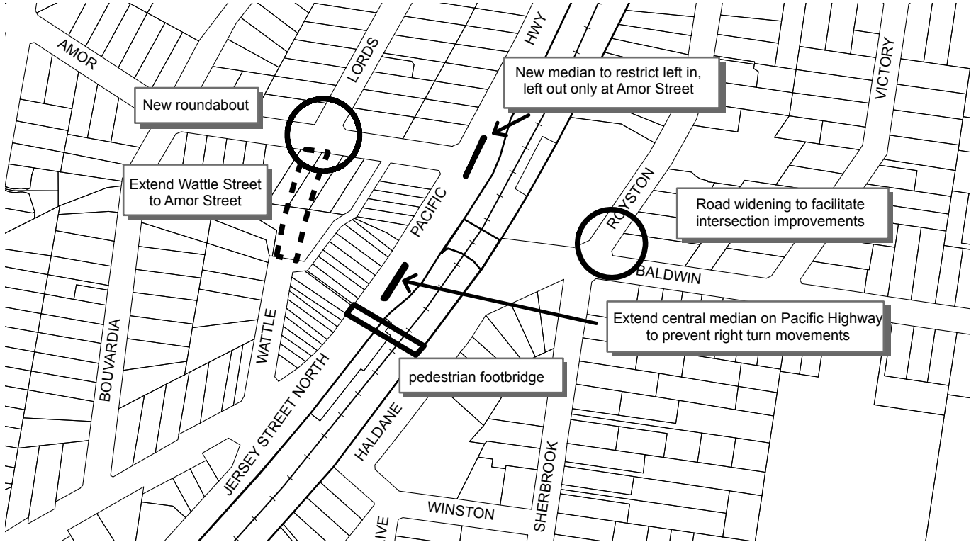
Figure 3.4(l): Traffic Management Improvement Plan - Asquith (C).
